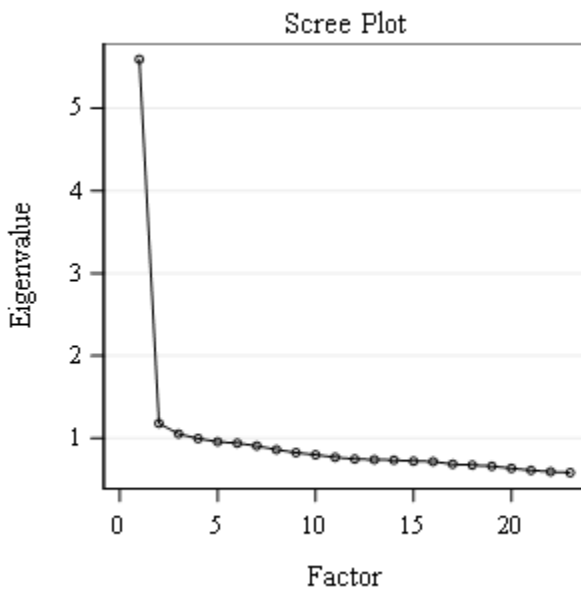
Figure I.6. Principal Component Scree Plot—Science Grade 10
