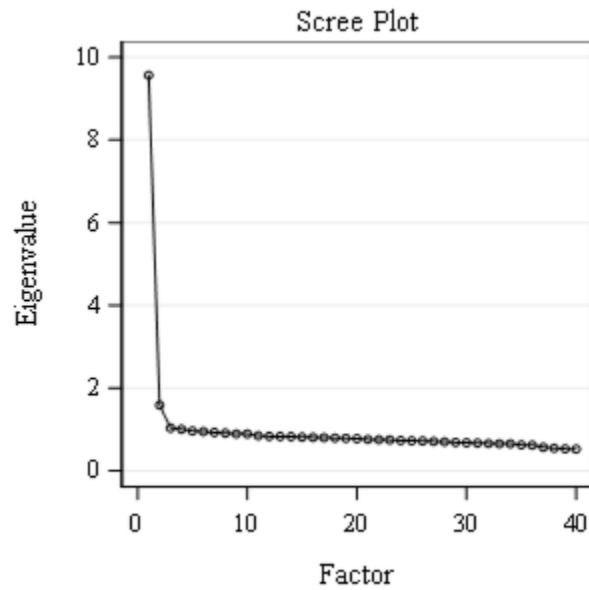
Figure I.3. Principal Component Scree Plot—Mathematics Grade 9
