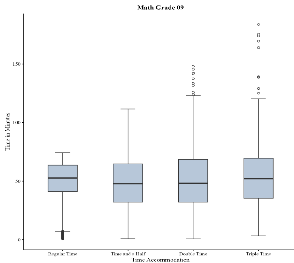
Figure B.3. Student Testing Time Plot—Mathematics Grade 9
